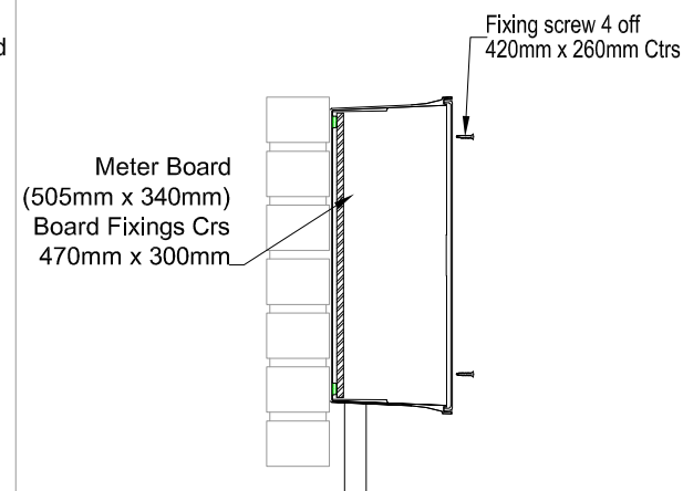
Surface Mounted Electricity Meter Box
