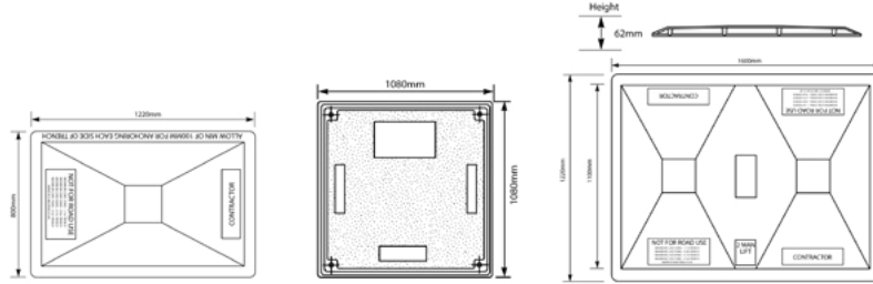
TRENCH COVER 1220X800MM 174001
